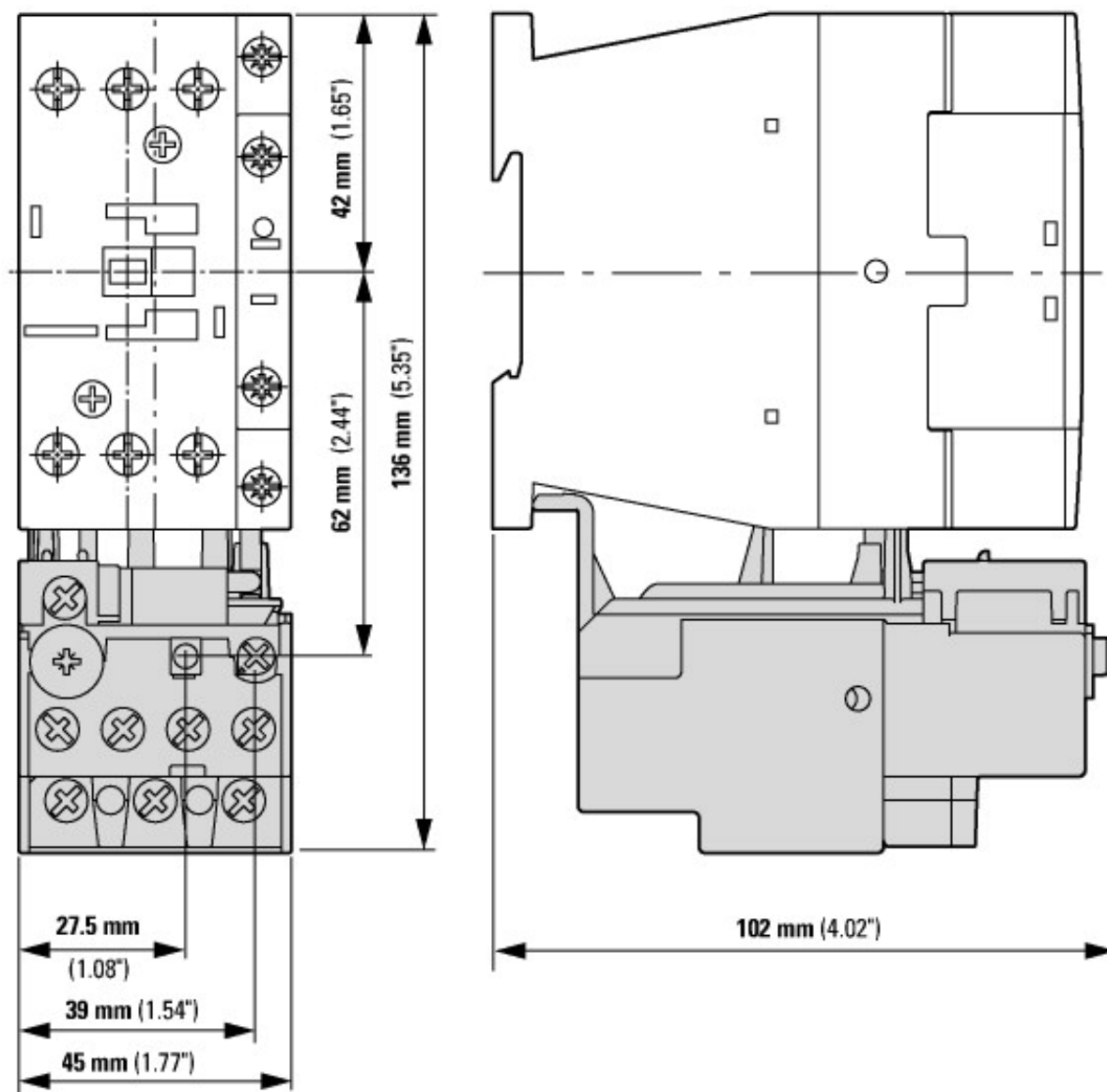
ZB32... + DILM
