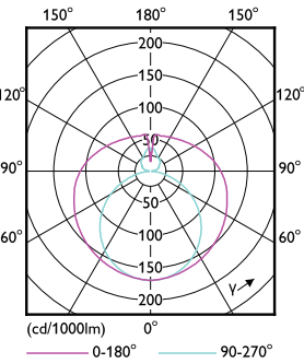
Light Distribution Diagram - MAS LEDtube VLE 1500mm HO 20.5W 830 T8
